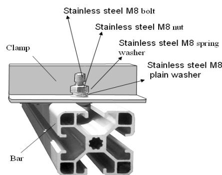
Fig. 8 Schematic diagram of the fringe clamp
