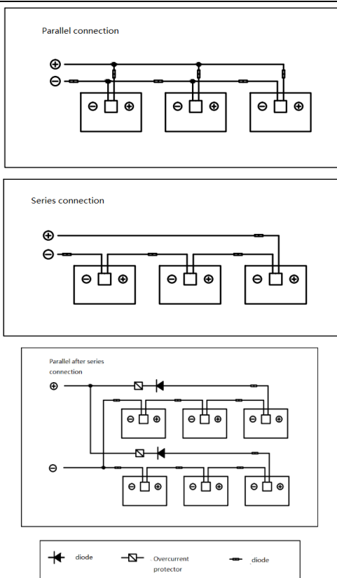
Fig. 17 Schematic diagram of electrical connection
