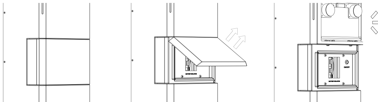
Fig. 15. HP-6S Magna-Flap & Installer Access Panel
